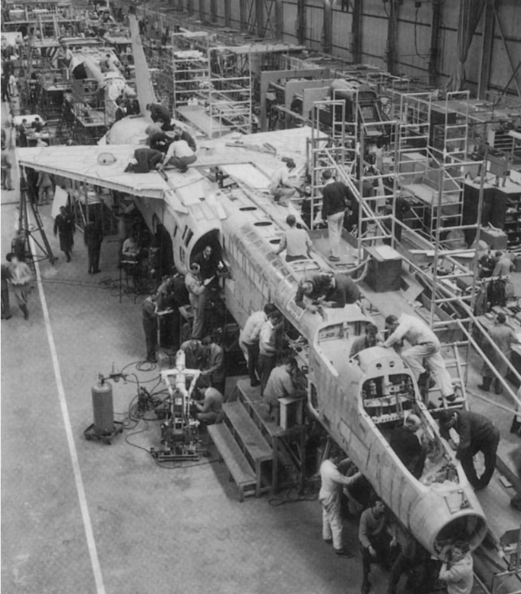
TSR2 under construction at Weybridge
