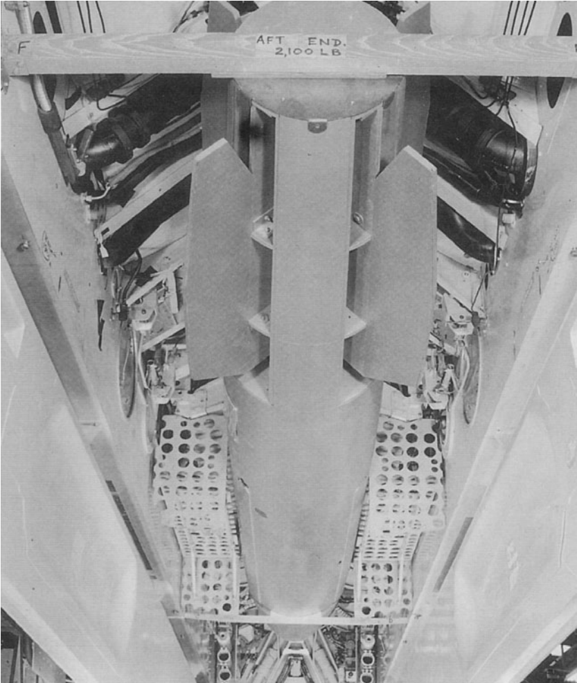
TSR2's weapons bay showing a mock-up 2,100 lb weapon
