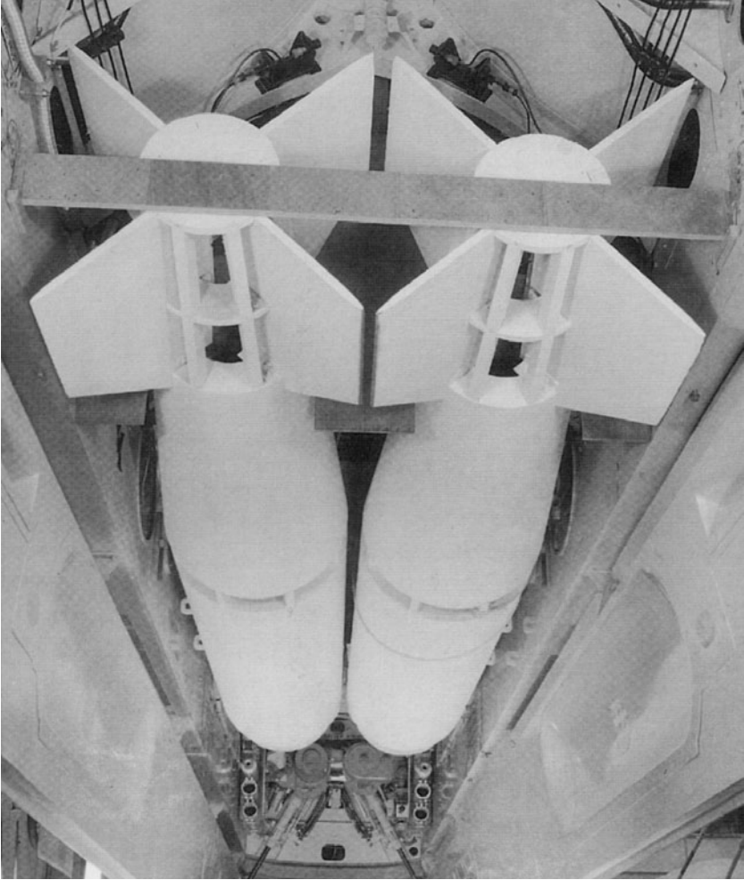
TSR2's weapons bay showing mock-up 1,000 lb bombs
