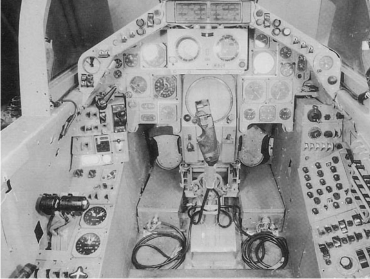
TSR2 front cockpit
